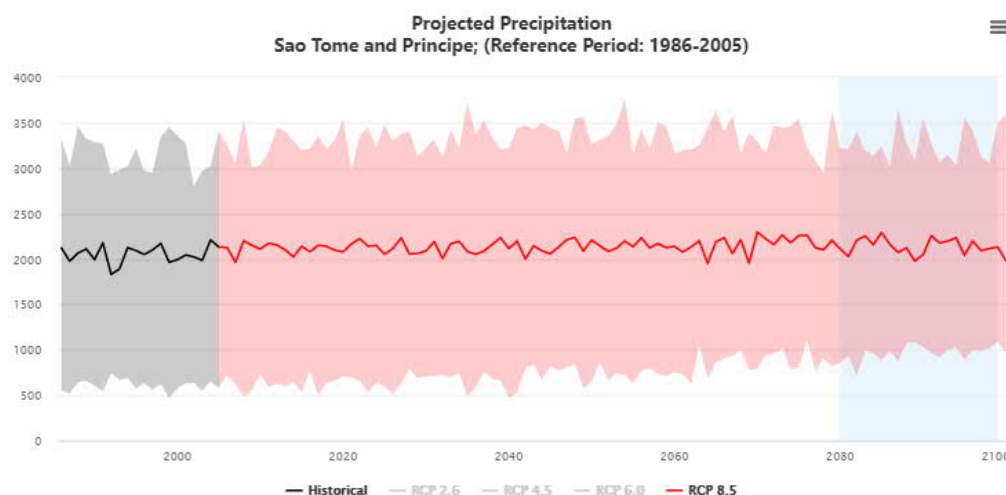
Figure 9 Projected precipitation evolution for the RCP 8.5 scenario in São Tomé and Príncipe (World Bank Climate Knowledge Portal)
