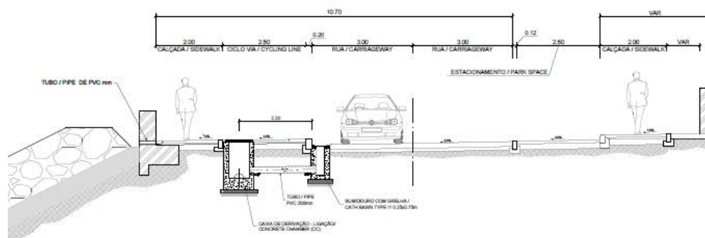
Figure 15 Typical section Lagarto bay with park space (0+000 – 1+880).
