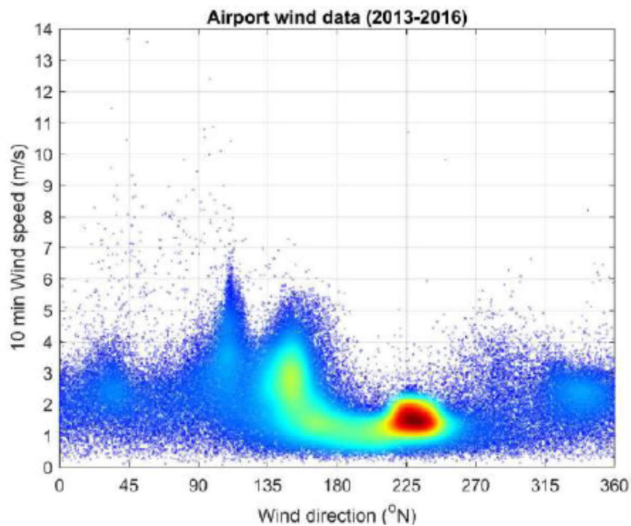
Figure 72 Wind direction and 10 min average wind speed scatter plot for airport wind data Source: CDR (2019)
