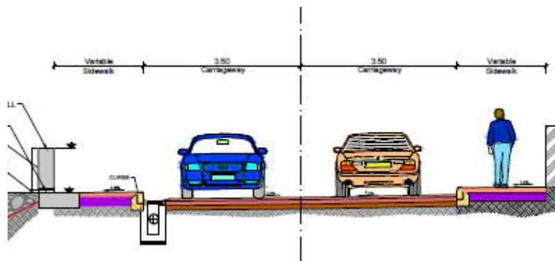
Figure 42 Typical section without cycle lane – Pantufo Coastline, São Tomé
