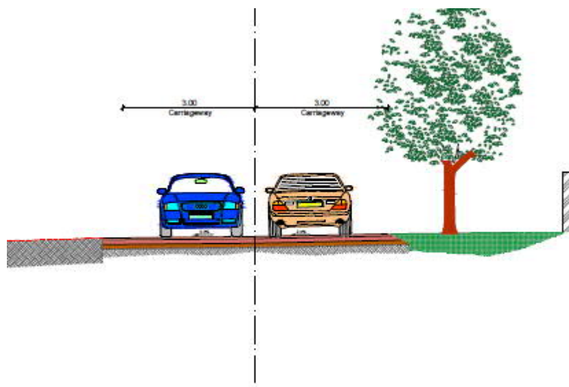
Figure 43 Typical section. Pantufo, Sao Tomé
