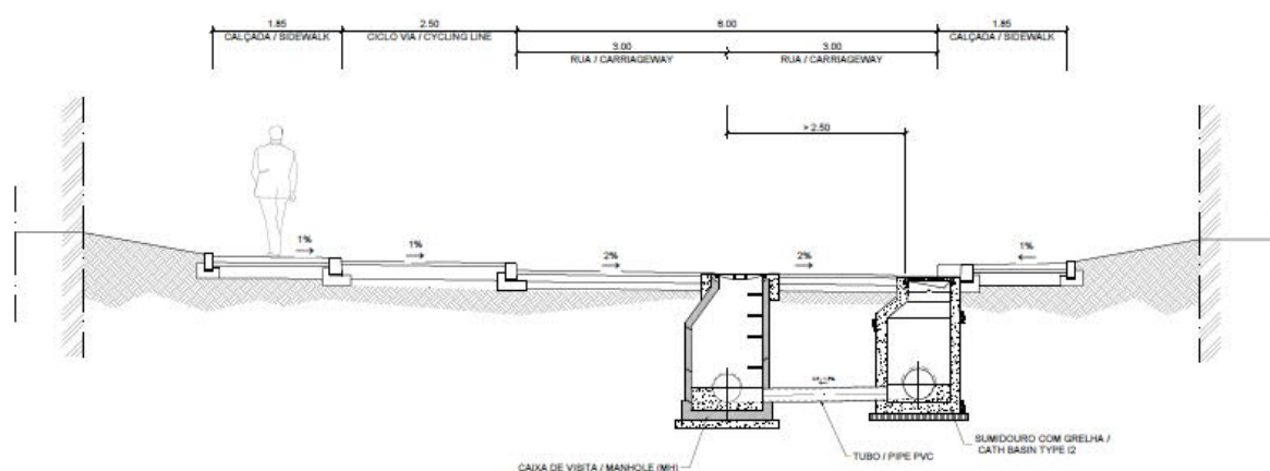
Figure 47 Typical section Pantufo Coastline (7+370 – 7+625).
