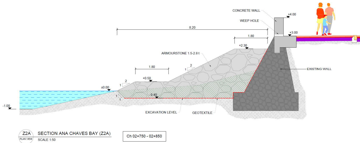
Figure 34: Typical cross section Z2A. Ana Chaves bay (CH 2+750 – CH 2+850)
