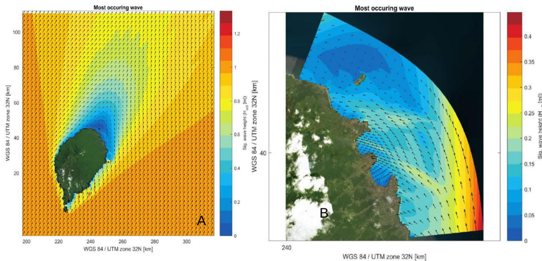
Figure 57 Wave propagation close to constant. A) comprehensive grid of the most frequent waves, B) detailed grid of waves close to the project's area of influence. Source: (CDR, 2019)
