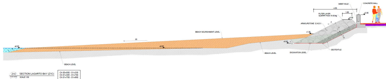
Figure 19 Typical cross section Z1C. Lagarto bay
