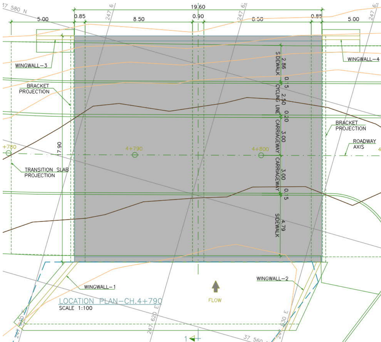
Figure 30 New structure proposed CH 4+790 (Ana Chaves bay)
