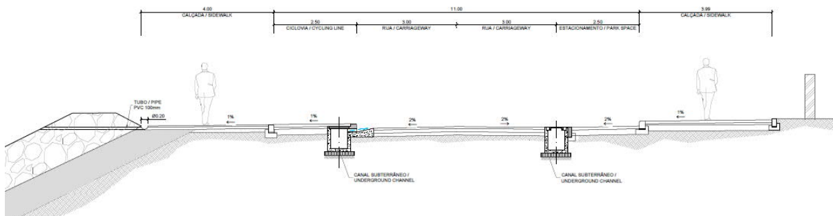
Figure 29 Typical section Ana Chaves bay (5+040 – 5+440).
