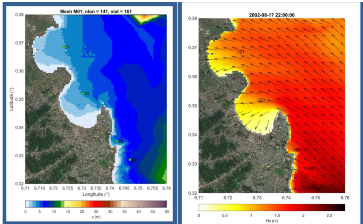
Figure 58 Point locations used to characterise the local wave climate and Significant Wave Height associated to the most energetic event in the project area with the selected points. Source: RD6767-DD-AN-CP-A5-Meteo-D01a
