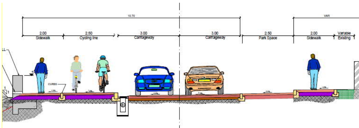
Figure 22 Typical section with parking – Ana Chaves, São Tomé
