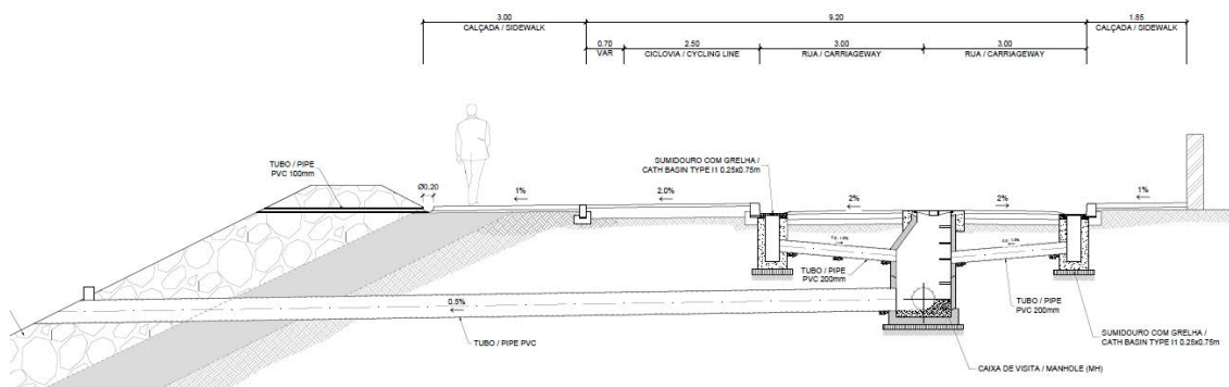
Figure 26 Typical section Ana Chaves bay without park space (2+760 – 4+520; 4+720 – 5+040; 5+440 – 5+900).
