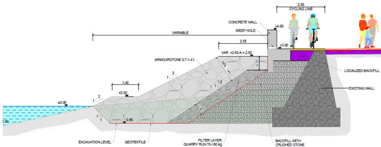
Figure 37: Typical cross section Z2D. Ana Chaves bay
