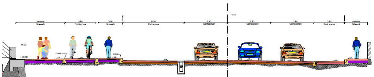
Figure 24 Typical section. Parking zone – Ana Chaves, Sao Tomé
