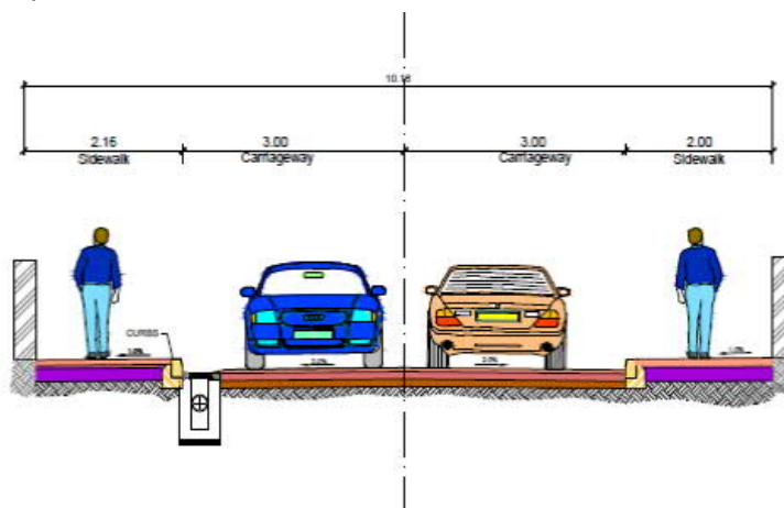
Figure 12 Typical section - Lagarto bay, Sao Tomé
