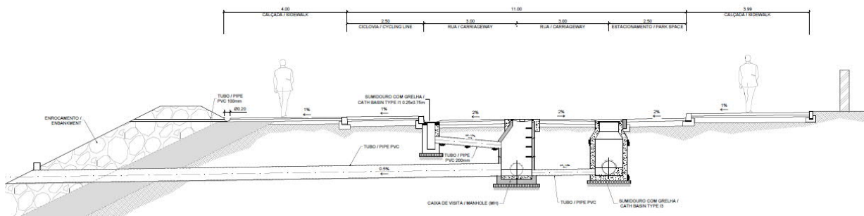
Figure 27 Typical section Ana Chaves bay with park space (2+760 – 4+520; 4+720 – 5+040; 5+440 – 5+900).
