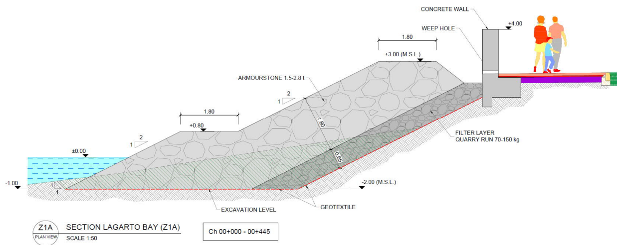
Figure 17 Typical cross section Z1A. Lagarto bay (CH 0+000 – 0+445)
