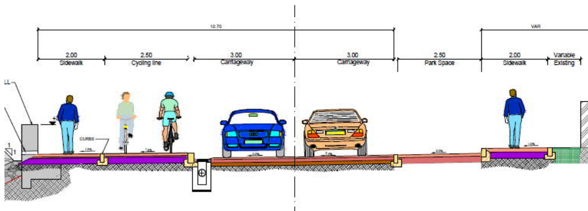
Figure 40 Typical section with parking – Pantufo Coastline, São Tomé
