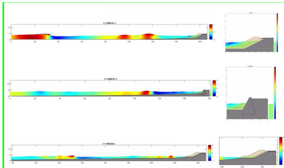
Figure 13 Output IH2VOF numerical simulation São Tomé Overtopping assessment
