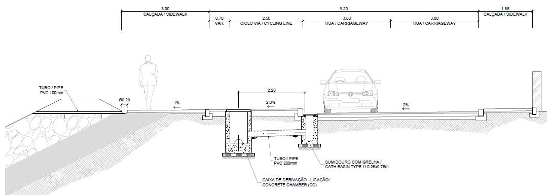
Figure 14 Typical section Lagarto bay without park space (0+000 – 1+880).
