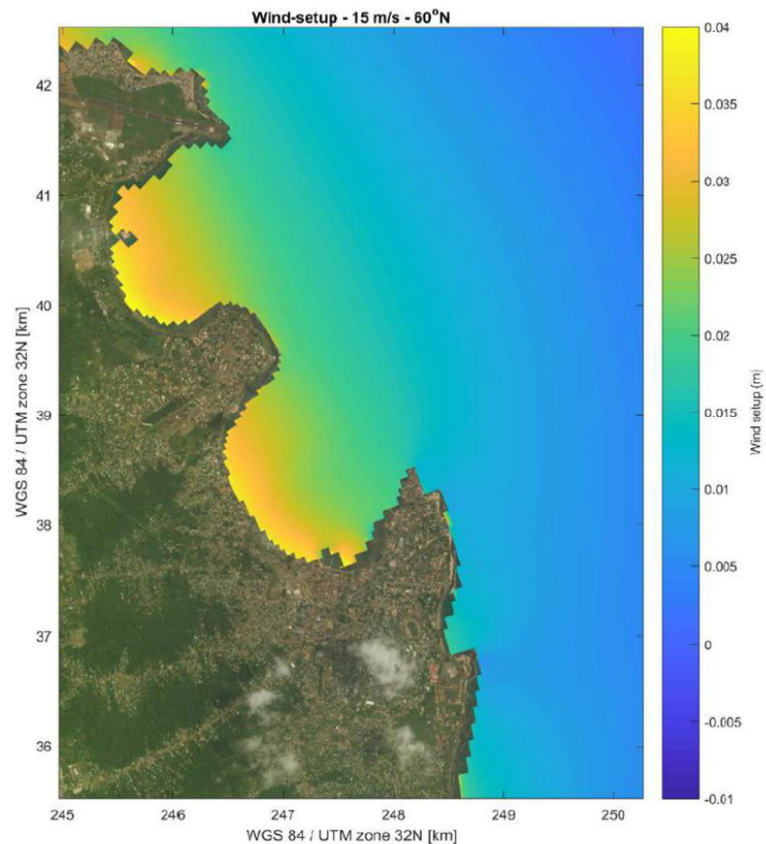
Figure 70 Wind setup for Return period of 100 years Source: CDR (2019)
