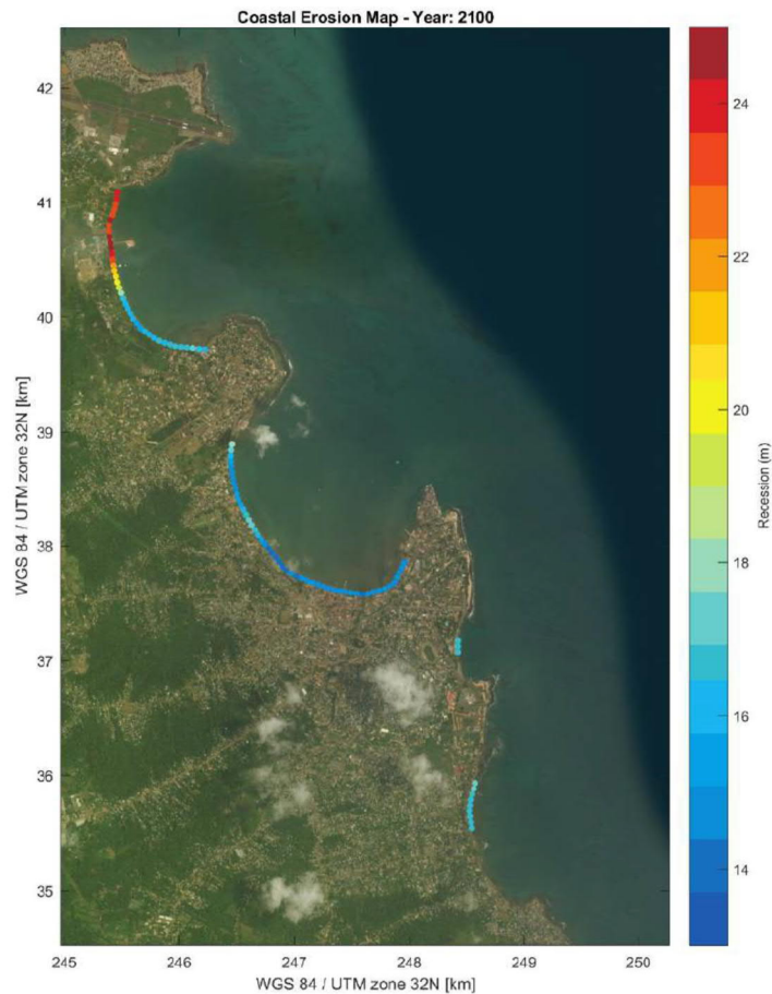
Figure 75 Potential coastal erosion due sea level rise for year 2100 Source: CDR (2019)
