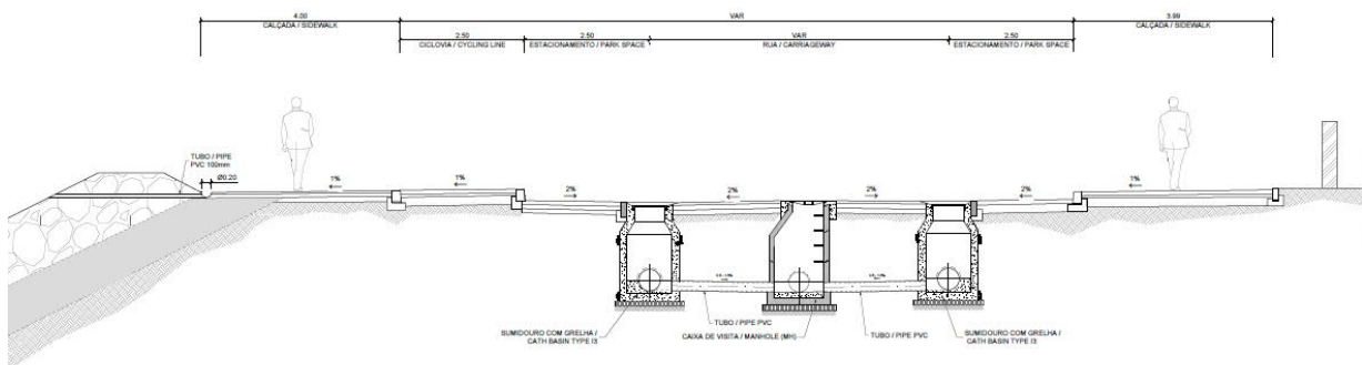
Figure 28 Typical section Ana Chaves bay (4+520 – 4+720).
