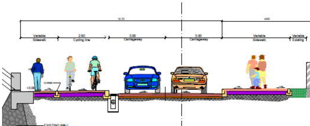
Figure 21 Typical section – Ana Chaves, São Tomé
