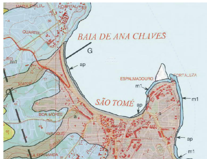
Figure 86 Geological map detail for Ana Chaves bay Section: From CH 2+760 to CH 5+800
