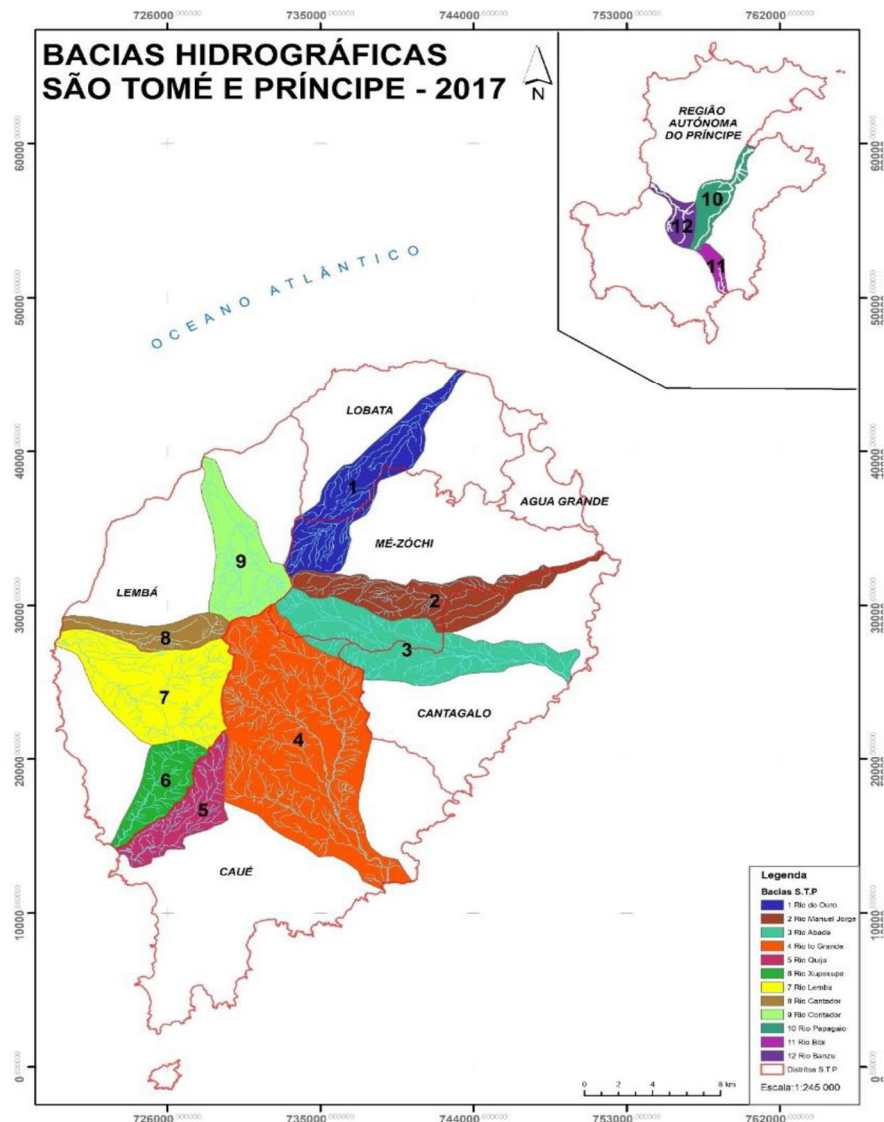
Figure 89 Main Hydrographic Basins of São Tomé and Príncipe. Source: Integrated Water Resources Management Implementation Plan, 2017
