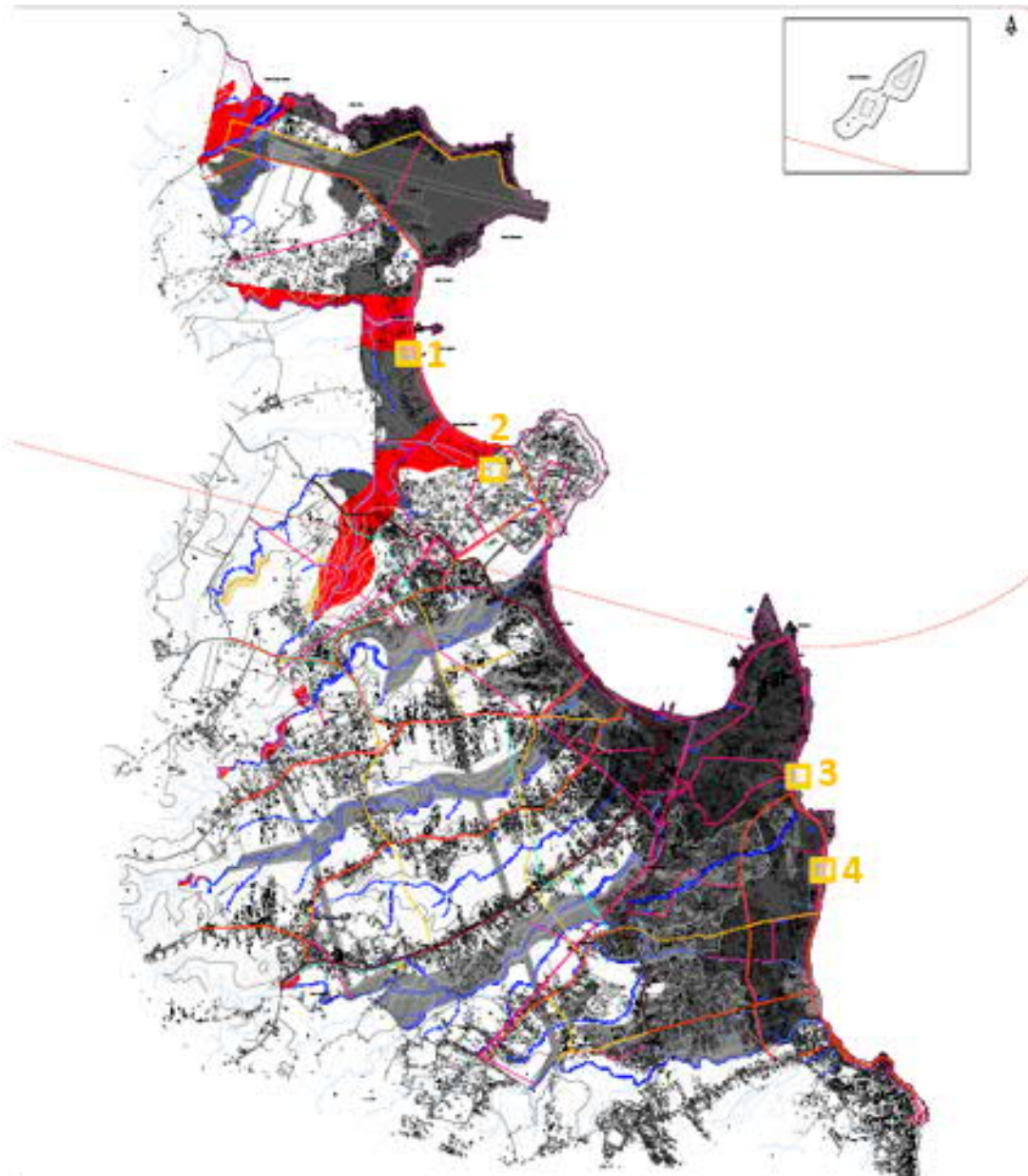
Figure 68 Hotels and flooding areas
