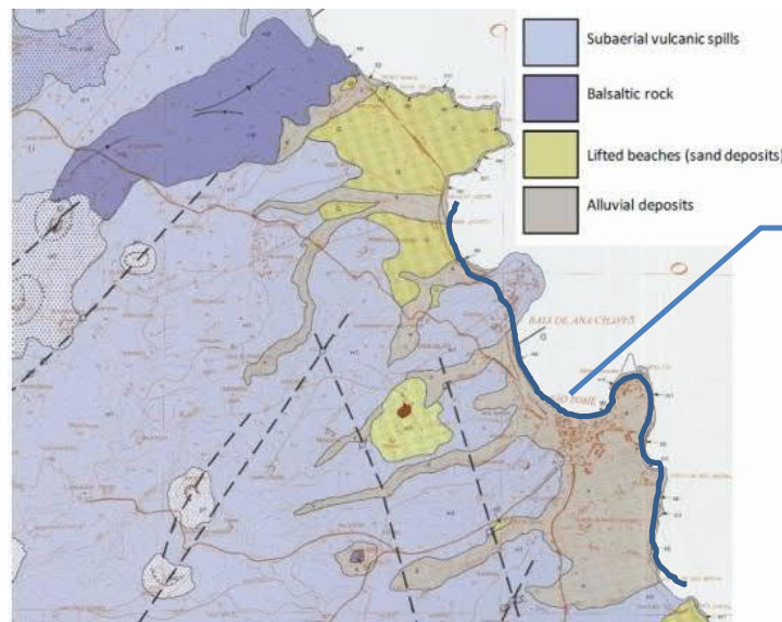
Figure 84 Geological map of Água Grande district
