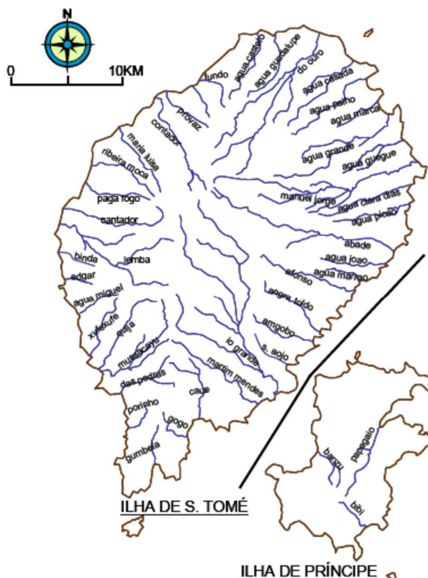
Figure 88 São Tomé and Príncipe's Hydrographic Network. Source: Global Water Resources Development Plan of S. Tomé & Príncipe, Nov 2009.
