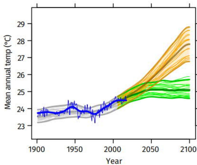
Figure 63 Mean annual temperature 1900-2100
