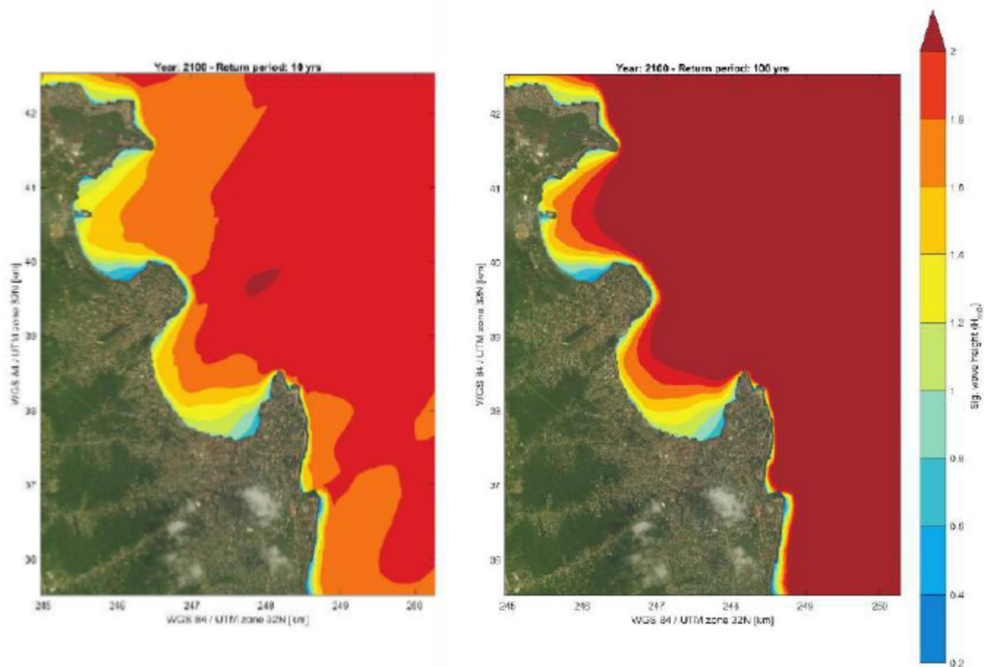
Figure 73 Extreme wind sea conditions year 2100 with a period of 10 years (left) and 100 years (right) Source: CDR (2019)
