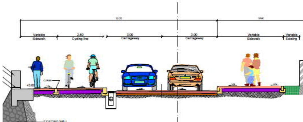
Figure 39 Typical section – Pantufo Coastline, São Tomé
