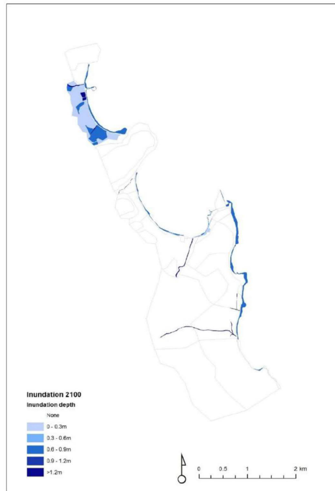
Figure 67 Inundation map for the year 2100 Source: CDR (2019)
