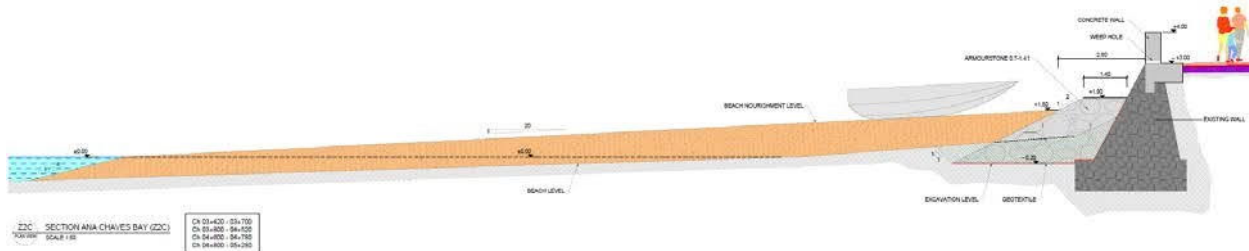
Figure 36: Typical cross section Z2C. Ana Chaves bay (CH 5+200 to CH 5+300)
