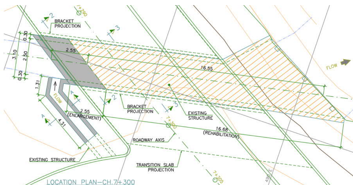
Figure 48 New structure proposed CH 7+300 (Pantufo Coastline)
