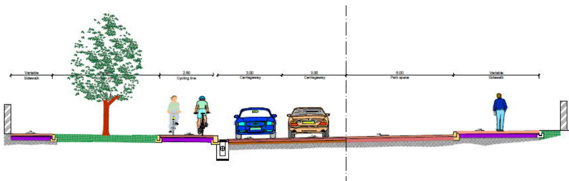
Figure 25 Typical section – Forte de São Sebastião, Sao Tomé
