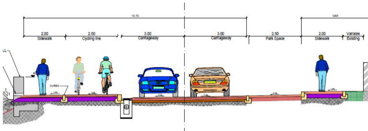
Figure 11 Typical section - Lagarto bay, Sao Tomé
