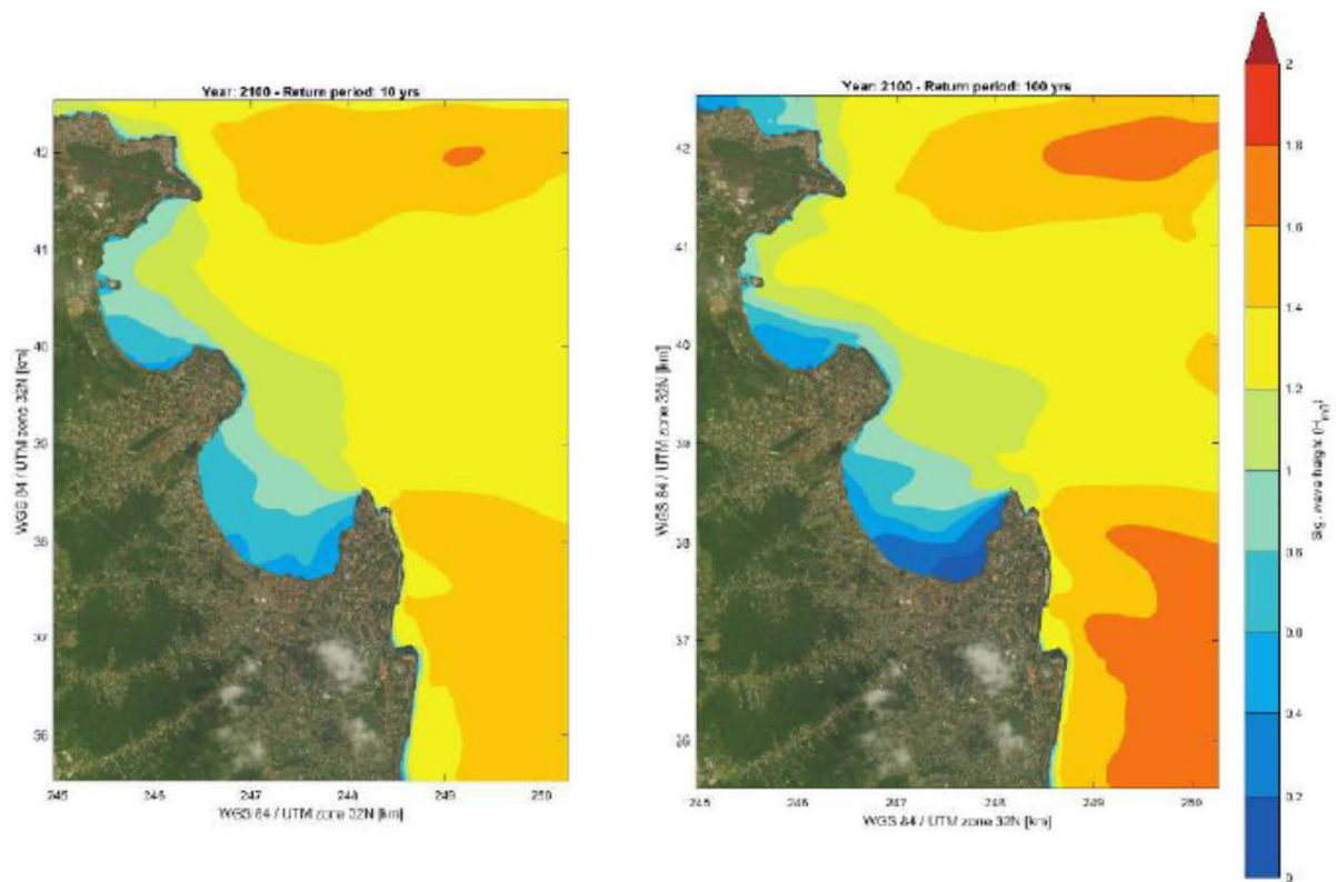
Figure 71 Extreme swell waves conditions for year 2100 with return period 10 years (left) and 100 years (right) Source: CDR (2019)
