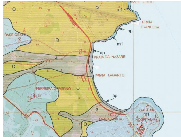
Figure 85 Geological map detail for Lagarto bay Section CH 0+000 - CH 2+760
