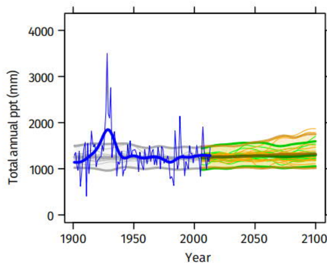
Figure 64 Total annual precipitation 1900-2100
