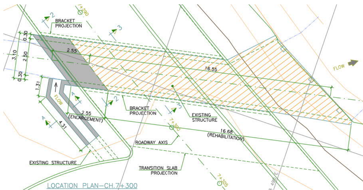
Figure 44 New structure proposed CH 7+300 (Pantufo Coastline)
