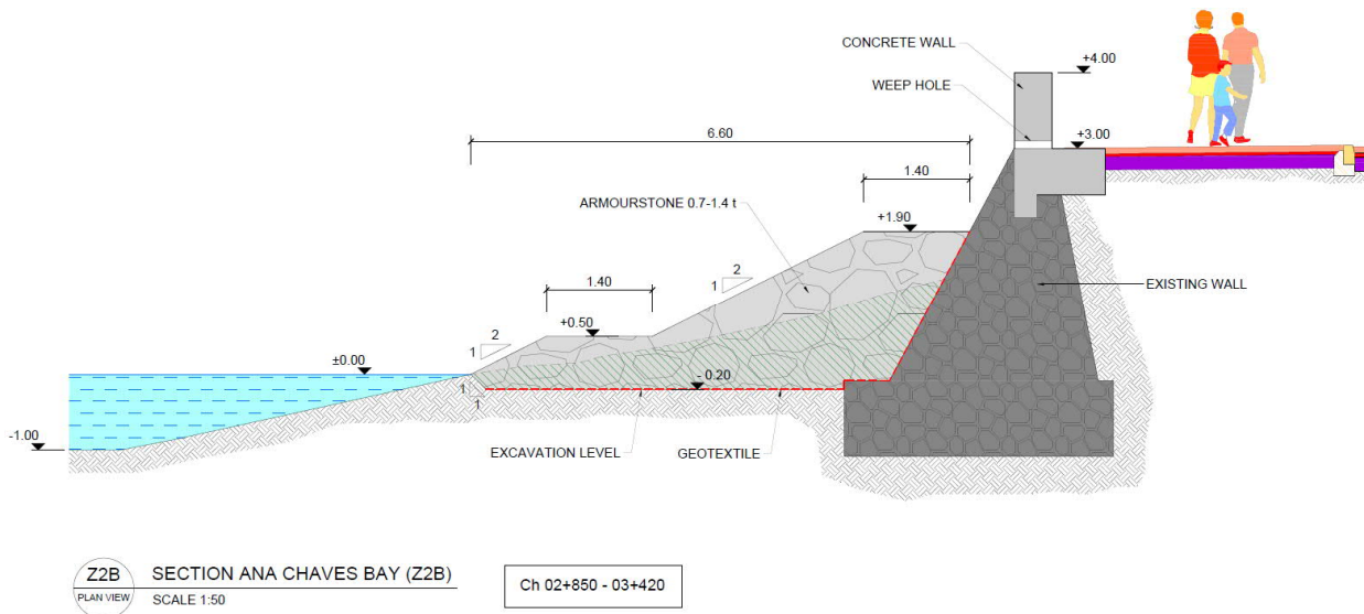
Figure 35: Typical cross section Z2B. Ana Chaves bay (CH 2+850 – CH 3+420)
