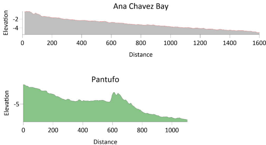
Figure 59 Cross-sections of the different zones. Source: bathymetric survey RD6767-DD-AN-CP-A2-BatSur-D01a.
