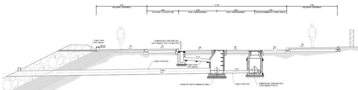
Figure 46 Typical section Pantufo Coastline with park space (5+900 – 7+370 and 7+625 – 7+660).
