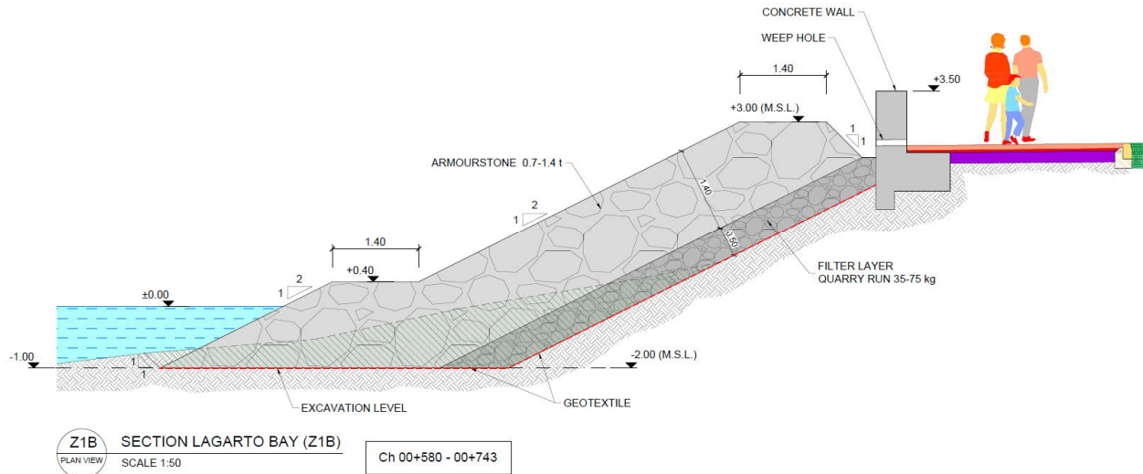
Figure 18 Typical cross section Z1B. Lagarto bay (CH 0+580 – CH 0+743)
