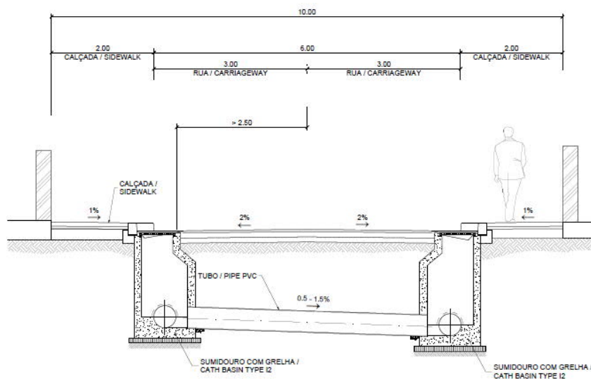
Figure 16 Typical section Lagarto bay (1+880 – 2+760).
