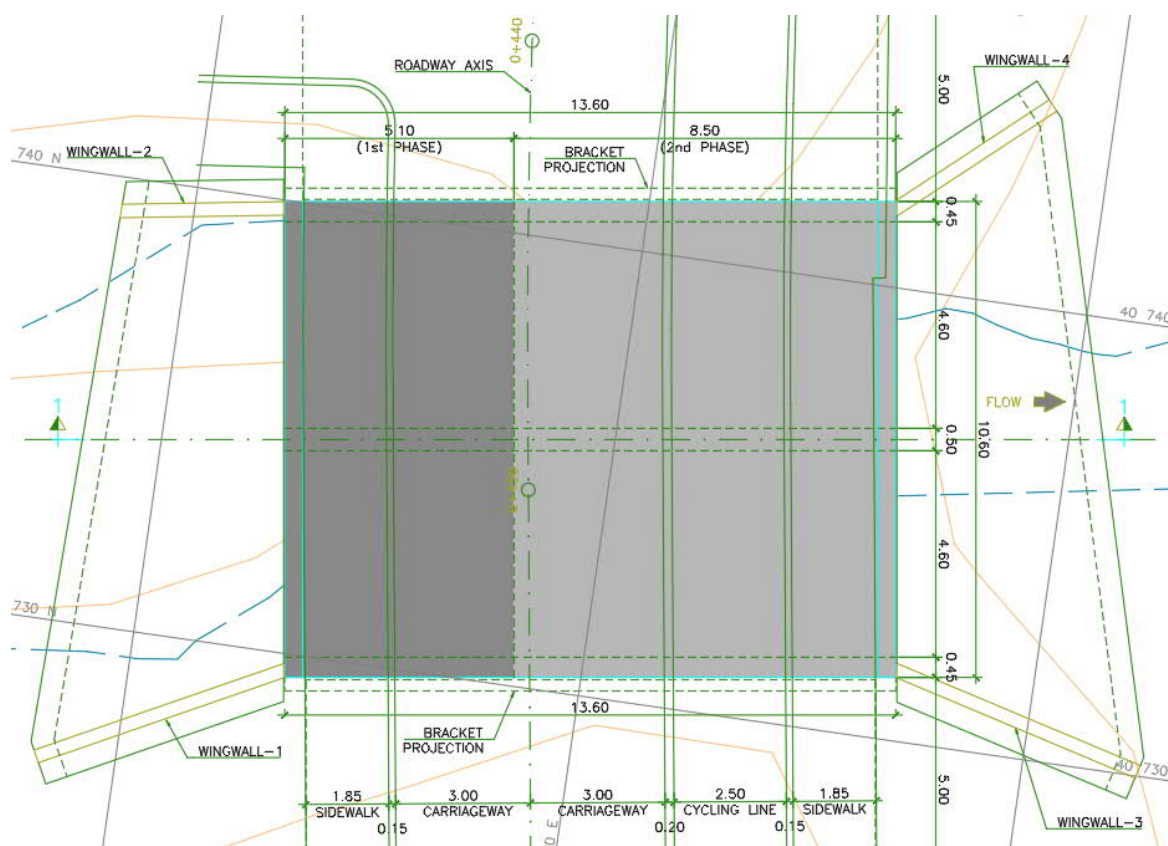
Figure 13 New structure proposed CH 0+450 (Lagarto bay)
