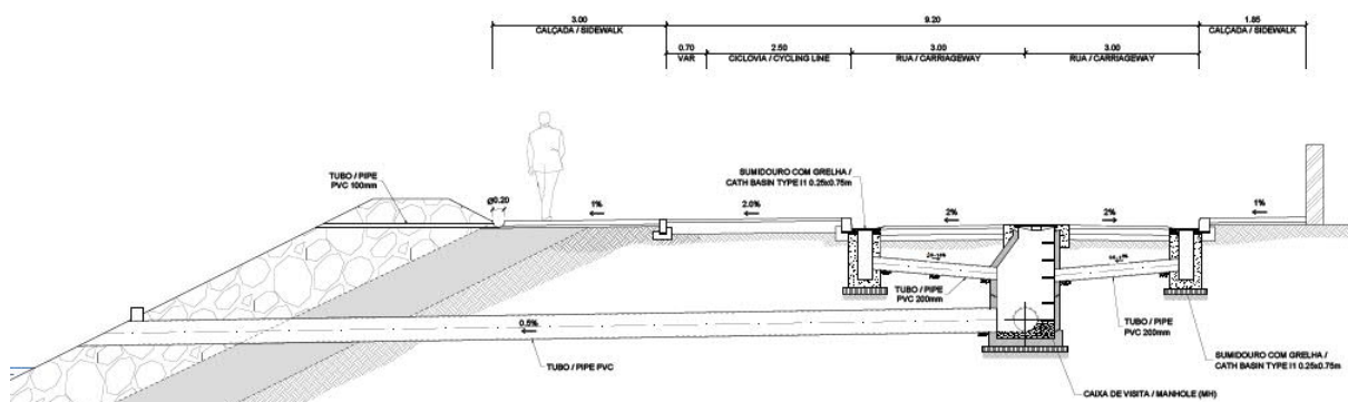
Figure 45 Typical section Pantufo Coastline without park space (5+900 – 7+370 and 7+625 – 7+660).
