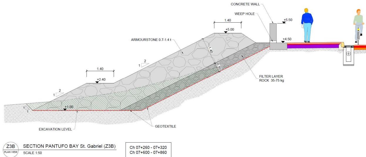
Figure 50 Typical cross section Z3B. Pantufo Coastline (CH 7+260 – CH 7+300; CH 7+600-CH 7+860)
