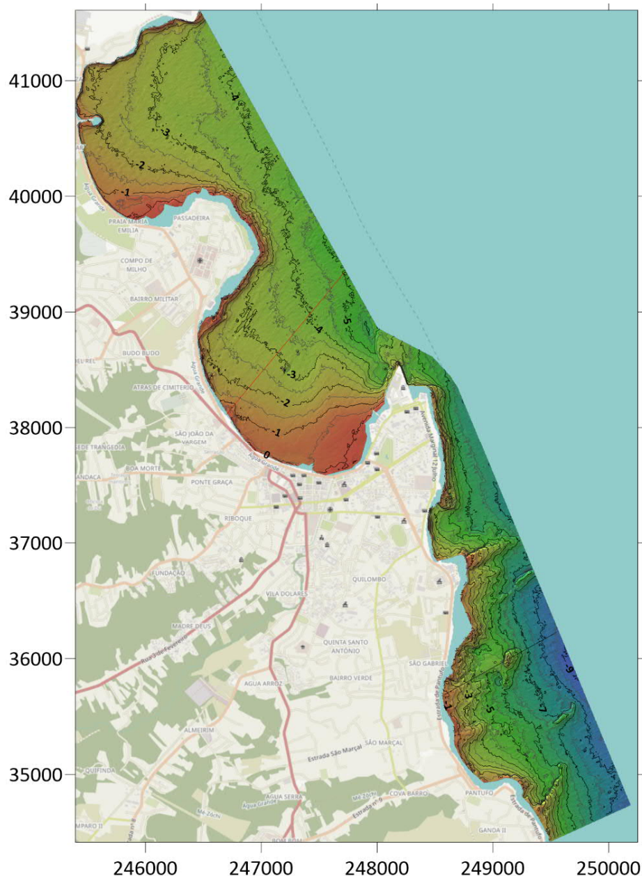
Figure 60 Contour map of the survey area. Source: Bathymetric Survey RD6767-DD-AN-CP-A2-BatSur-D01a
