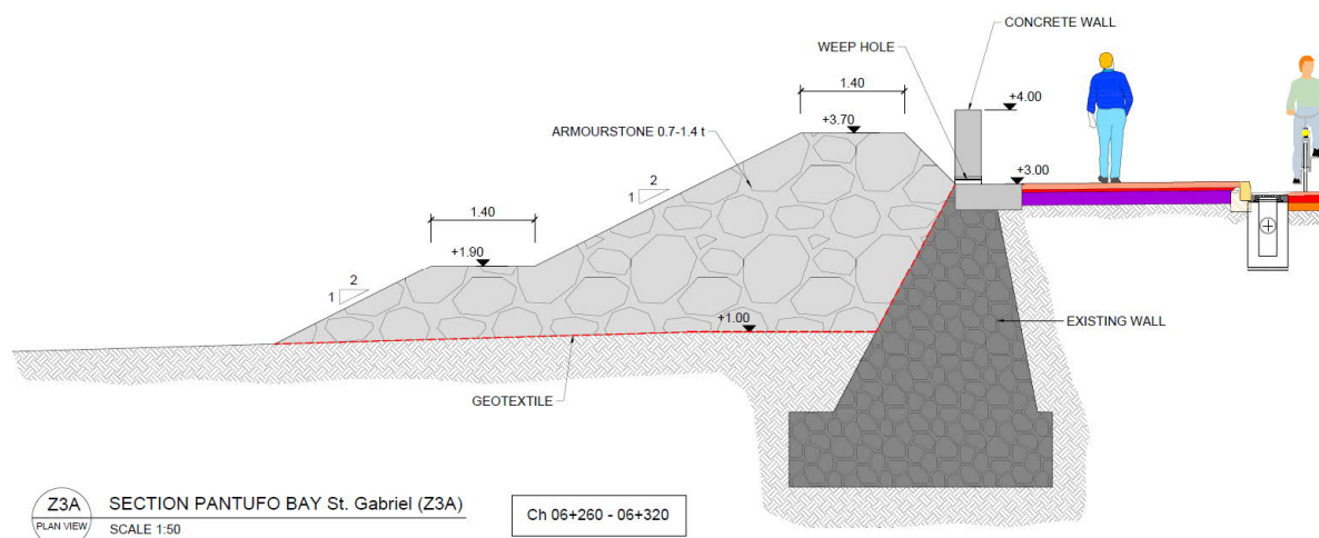
Figure 49 Typical cross section Z3A. Pantufo Coastline (CH 6+260 – CH 6+320)
