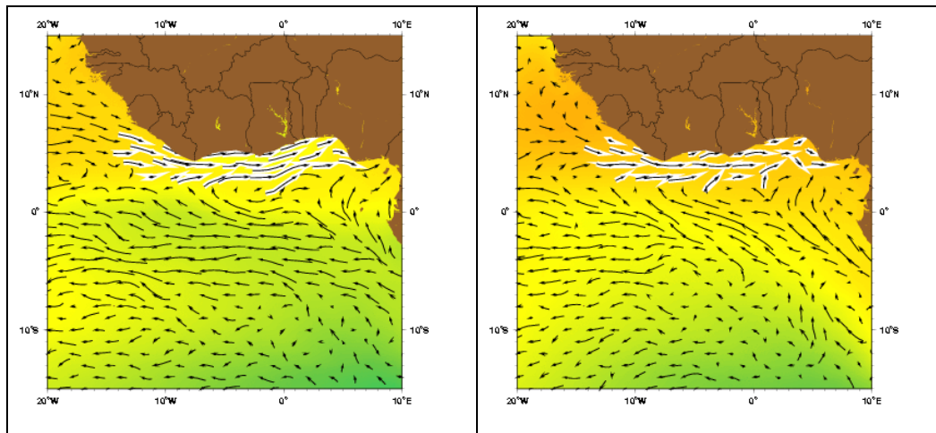
Figure 56 Mean Annual and seasonal directions of the Guinea and Benguela Currents (CGG, 2017)
