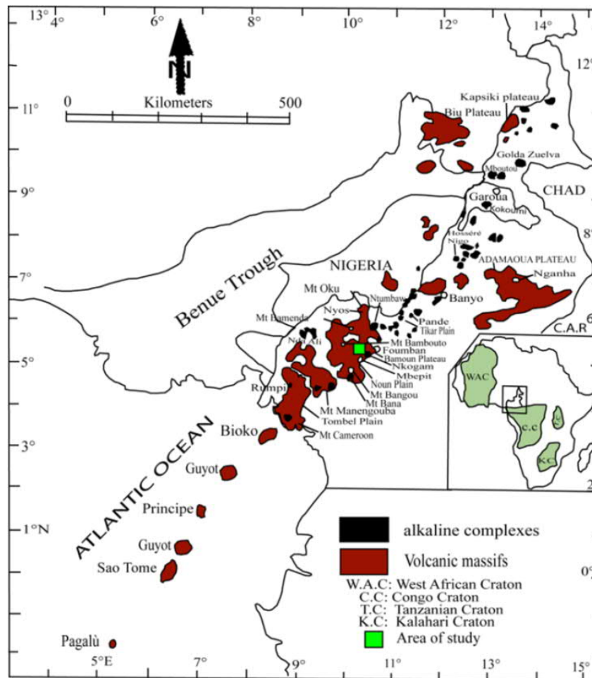
Figure 83 Alignment of the Cameroon Volcanic. Source VERIF-I (2017):
