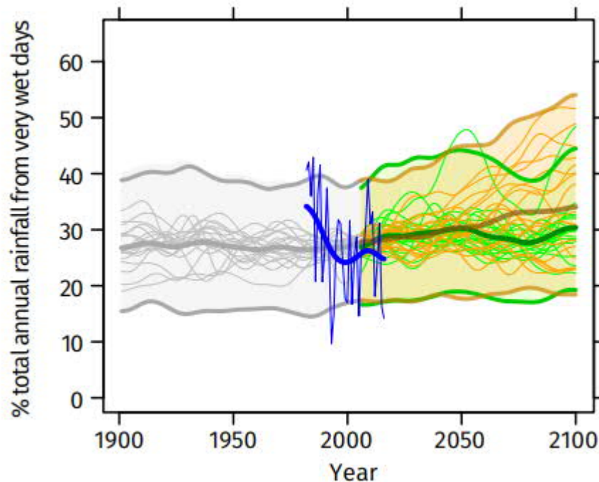
Figure 65 Contribution to total annual rainfall from very wet days ('extreme rainfall' and 'flood risk'), 1900–2100
