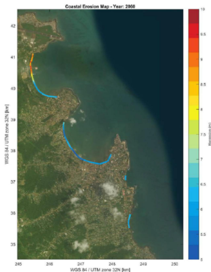
Figure 74 Potential coastal erosion due sea level rise for year 2060 Source: CDR (2019)
